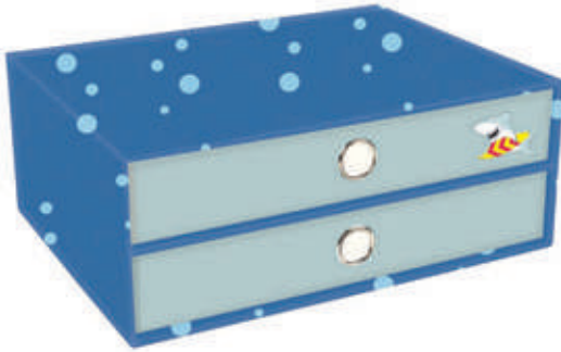
SHARK
